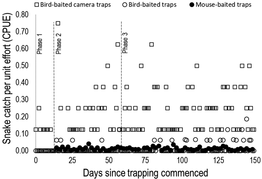
Figure 2. Brown treesnake catch per unit effort (CPUE) per trap night for bird-lure camera traps and bird- and mouse-lure live traps from 08 May through 05 October 2014 on the Guam National Wildlife Refuge, Guam. Open squares represent capturing a photographic image of the snake. Open and closed circles represent actual successful snake captures from traps. Phase I = only bird-lure traps deployed, Phase II = both bird- and mouse-lure traps deployed, and Phase III = both bird- and mouse-lure traps deployed with snake removal from mouse-lure traps only. Cameras were deployed on bird-lure traps during all three phases.
